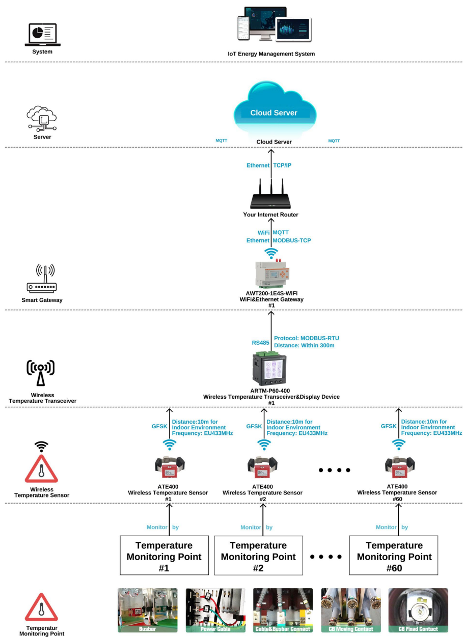
(1) Communication Structure
