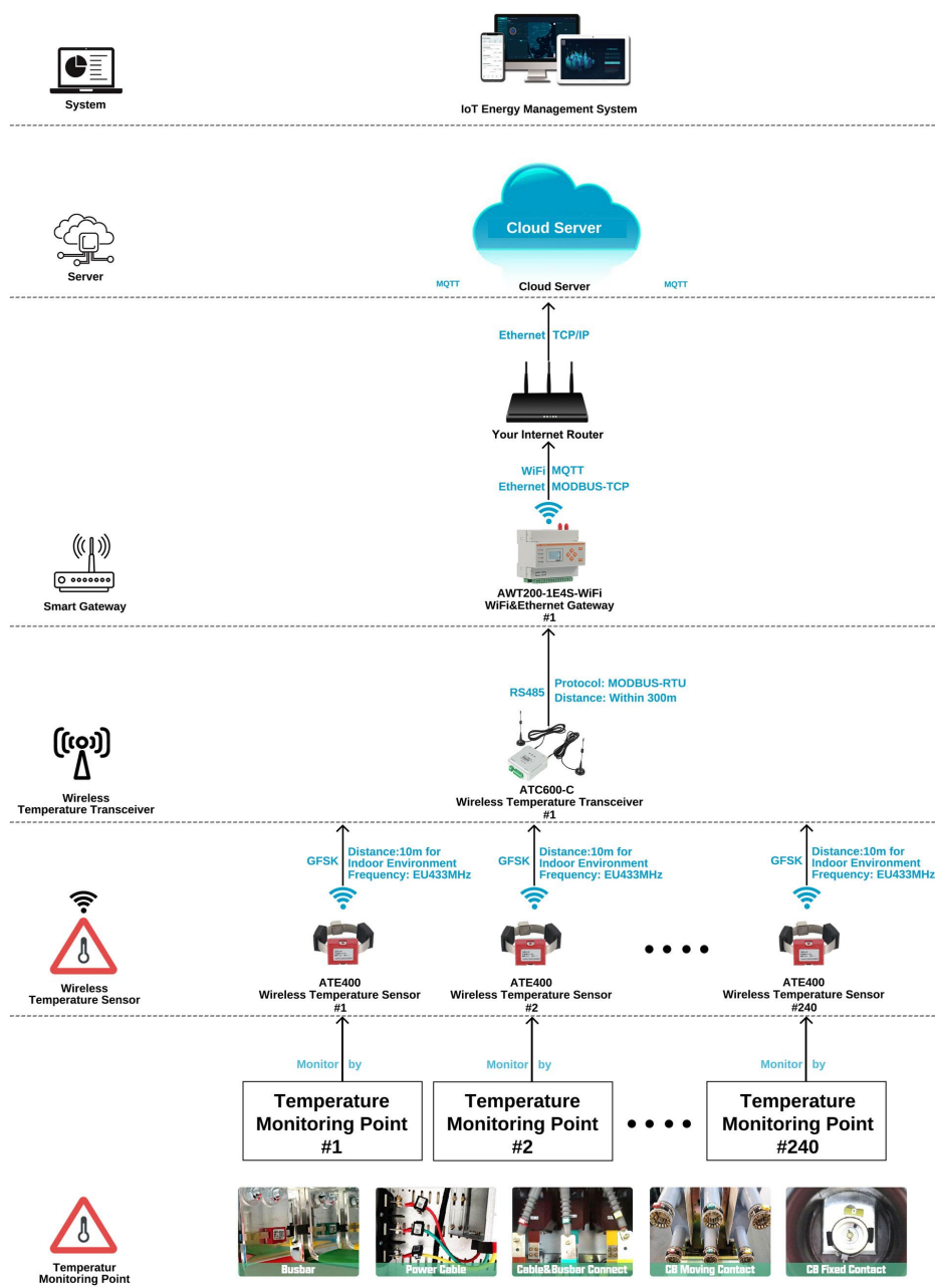
(1) Communication Structure
