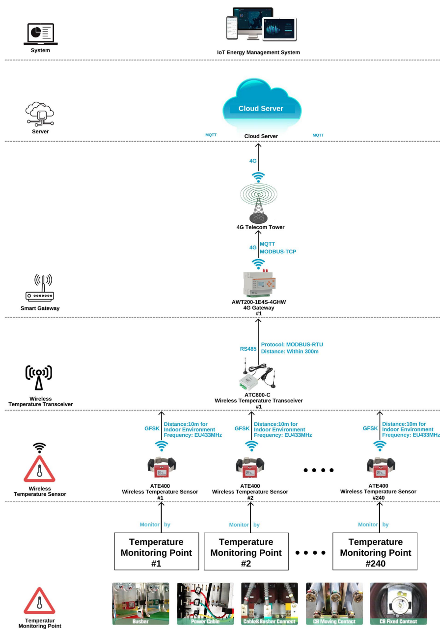
(1) Communication Structure
