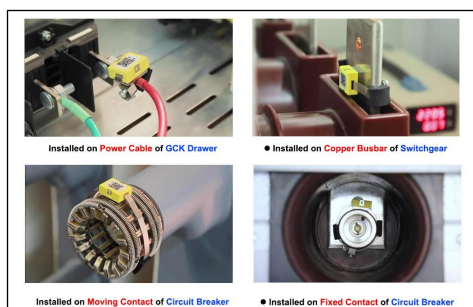
Switchgear Temperature Monitoring Point Showcase
