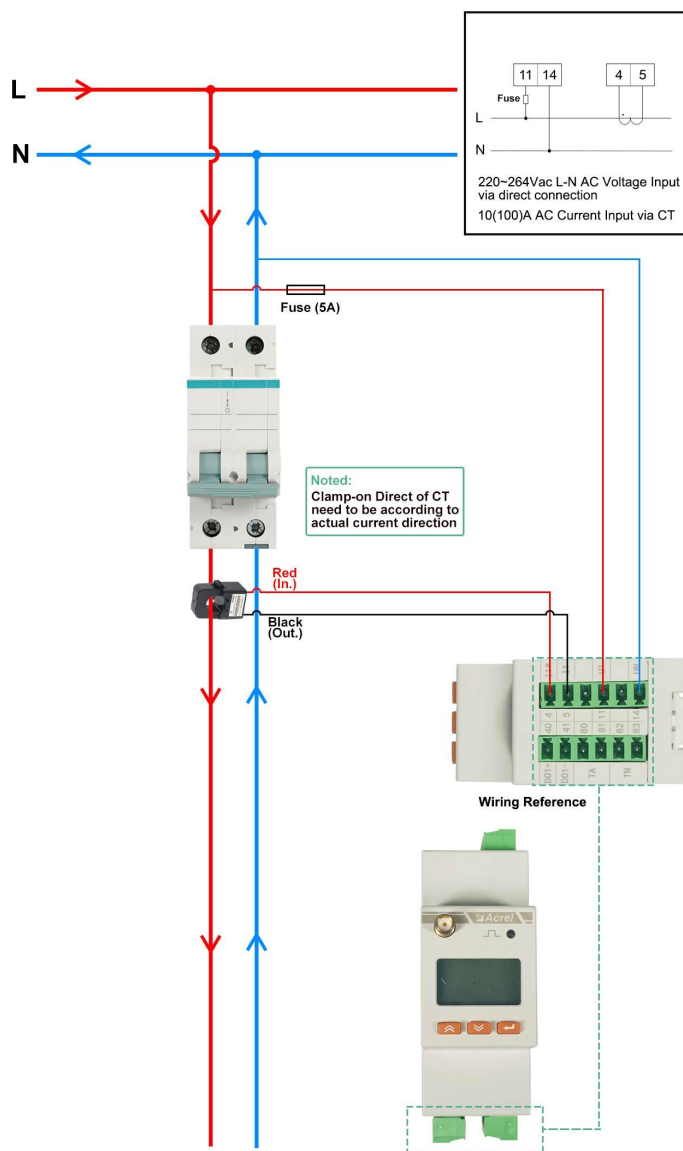
Current&Voltage Input Wiring of ADW310
